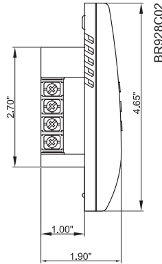
Dimensions (inch.)
